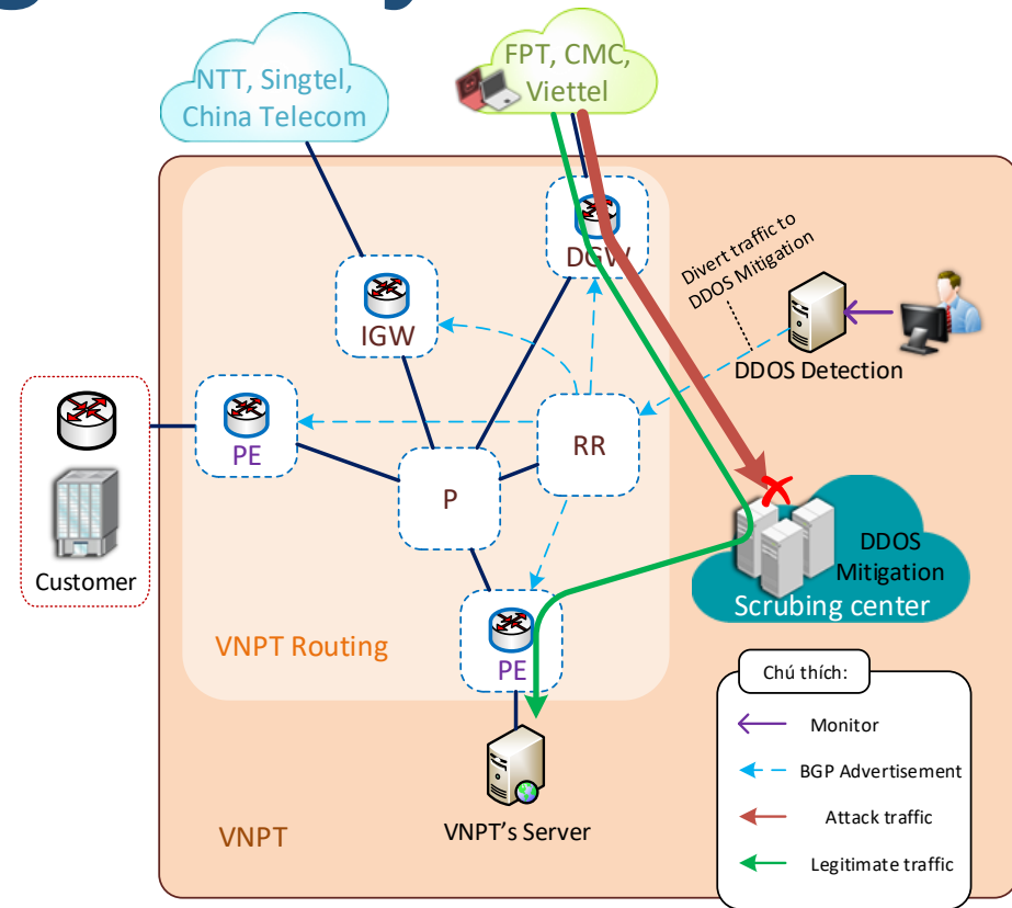
VNPT's DDoS system
