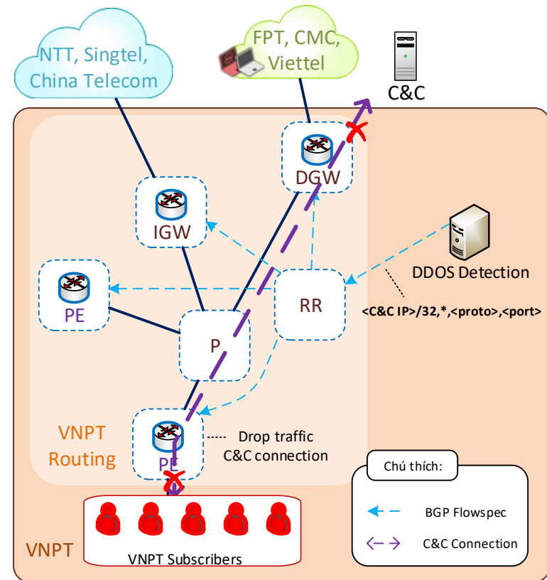
Block C&C connections using BGP flowspec
